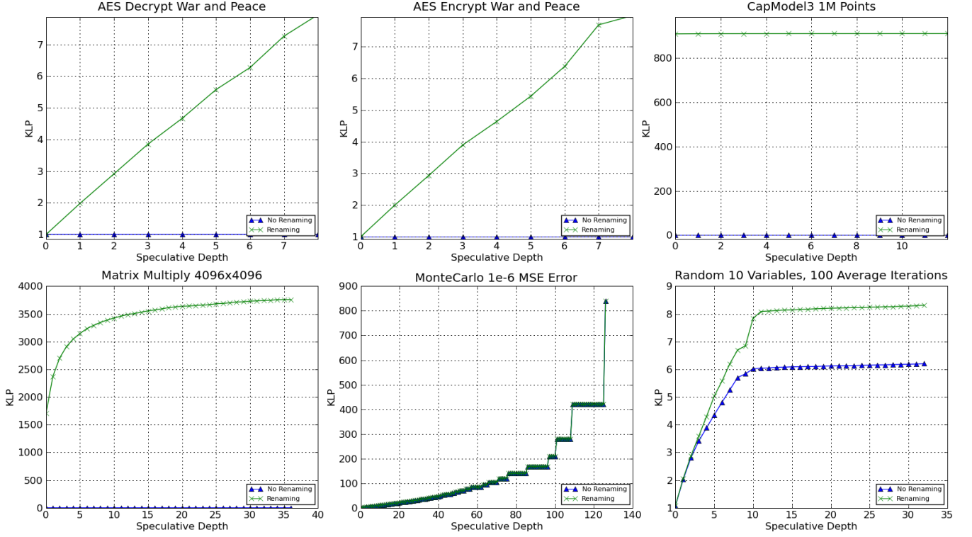
Fig. 6. Kernel Level Parallelism in Harmony Applications
