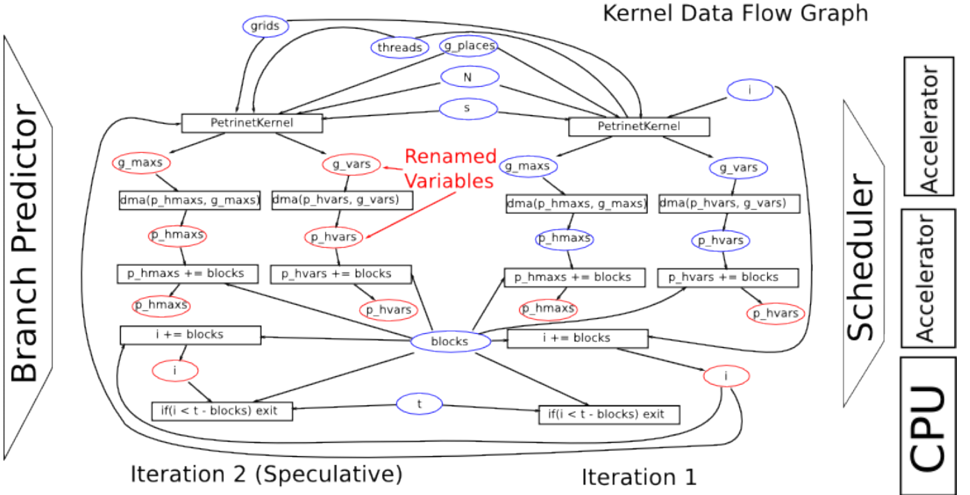
Fig. 5. Execution of a Harmony Application
