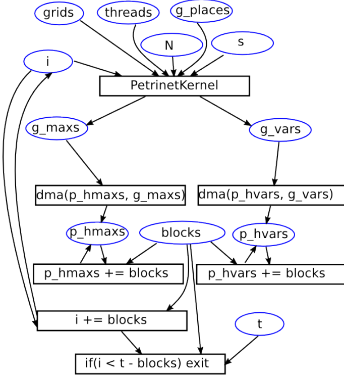
Fig. 3. Data Flow Graph for PNS Inner Loop
