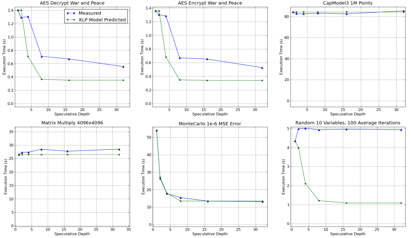
Fig. 8. KLP Predicted vs Measured Scaling (4 CPUs)
