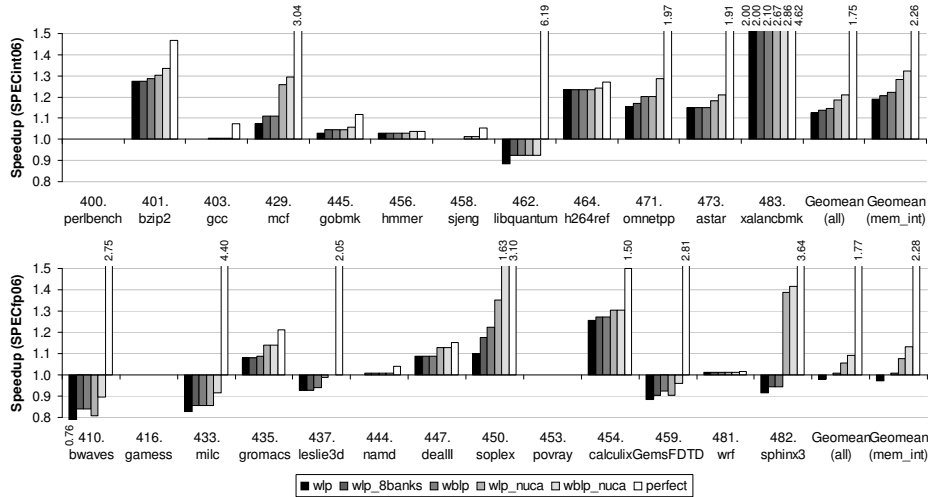
Figure 14: Relative Performance of Different C-Mode Designs
