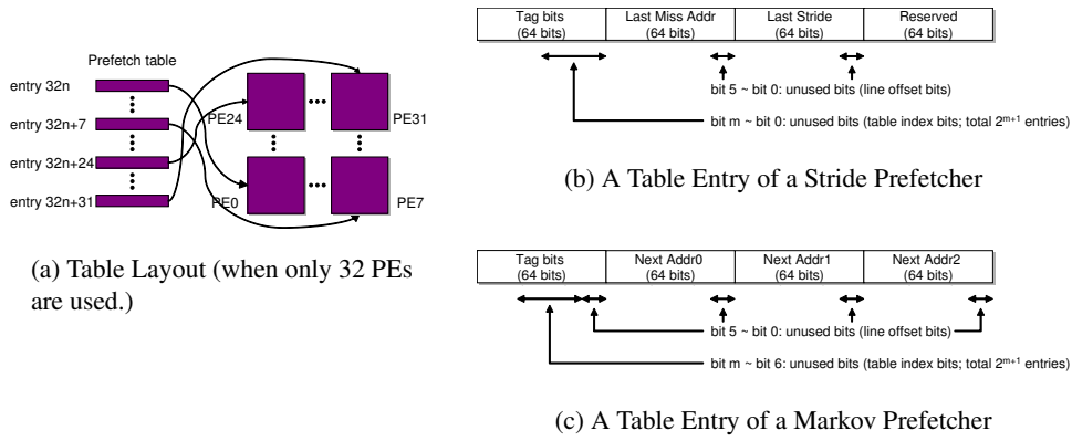
Figure 11: P-Mode Prefetcher
